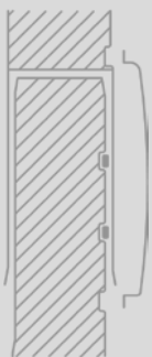
Male-Female push fit connection with external gaskets, secured by locking band 2.0
